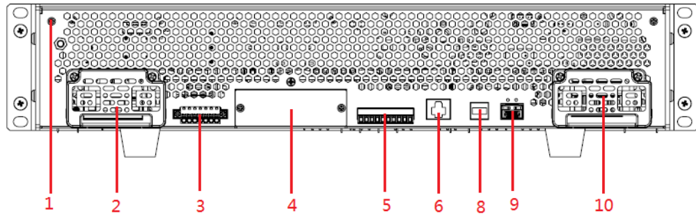
3U model rear panel illustration.
