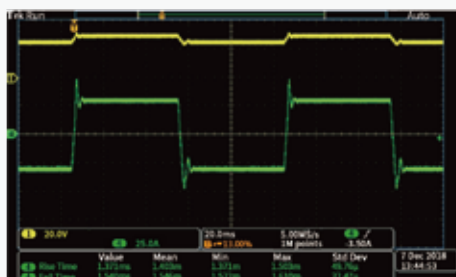
Control loop CV priority mode
